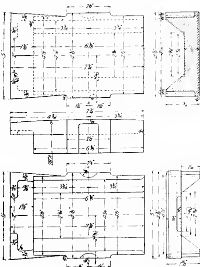
Figs. 5406-5410. WEDGE.
